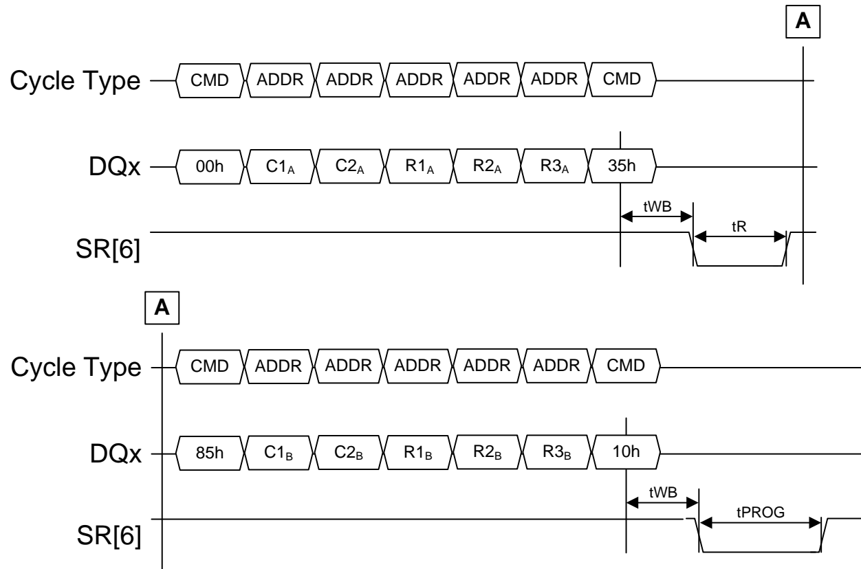
Figure 100 Copyback timing
