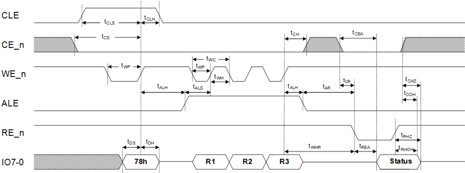
Figure 59 Read Status Enhanced timings
