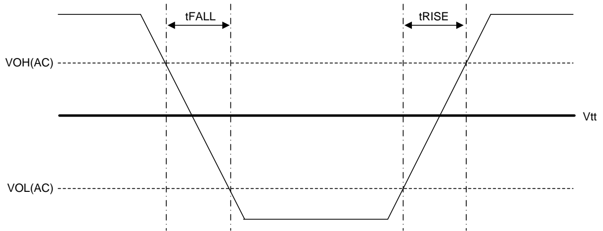
Figure 40 t_{RISE} and t_{FALL} Definition for Output Slew Rate, NV-DDR2 (single-ended)
