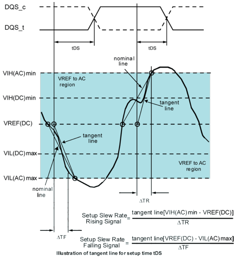
Figure 44 Tangent Line for Data Setup Time (tDS)
