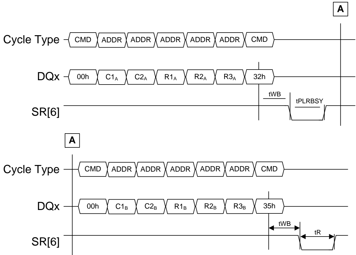
Figure 121 Multi-plane Copyback Read timing for Multi-plane Copyback Program
