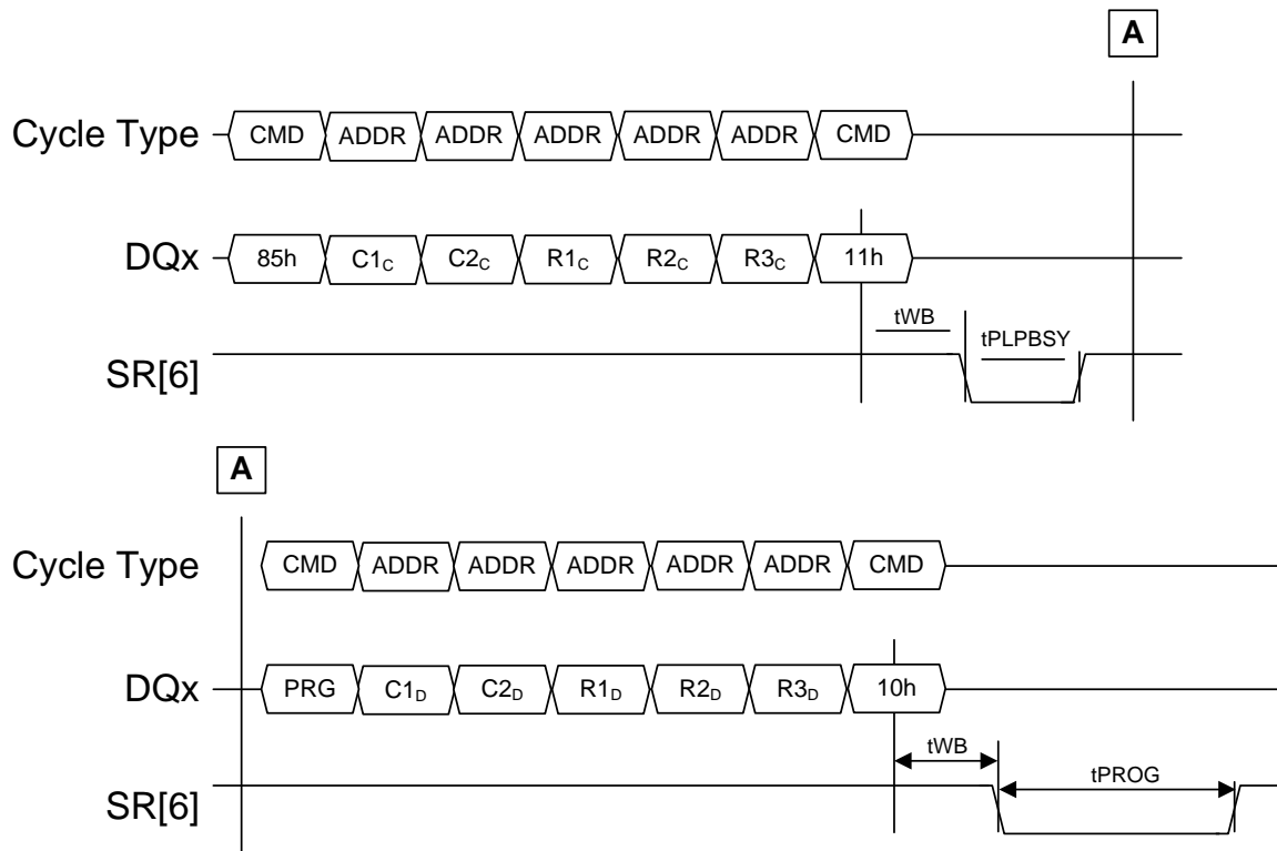
Figure 122 Multi-plane Copyback Program
