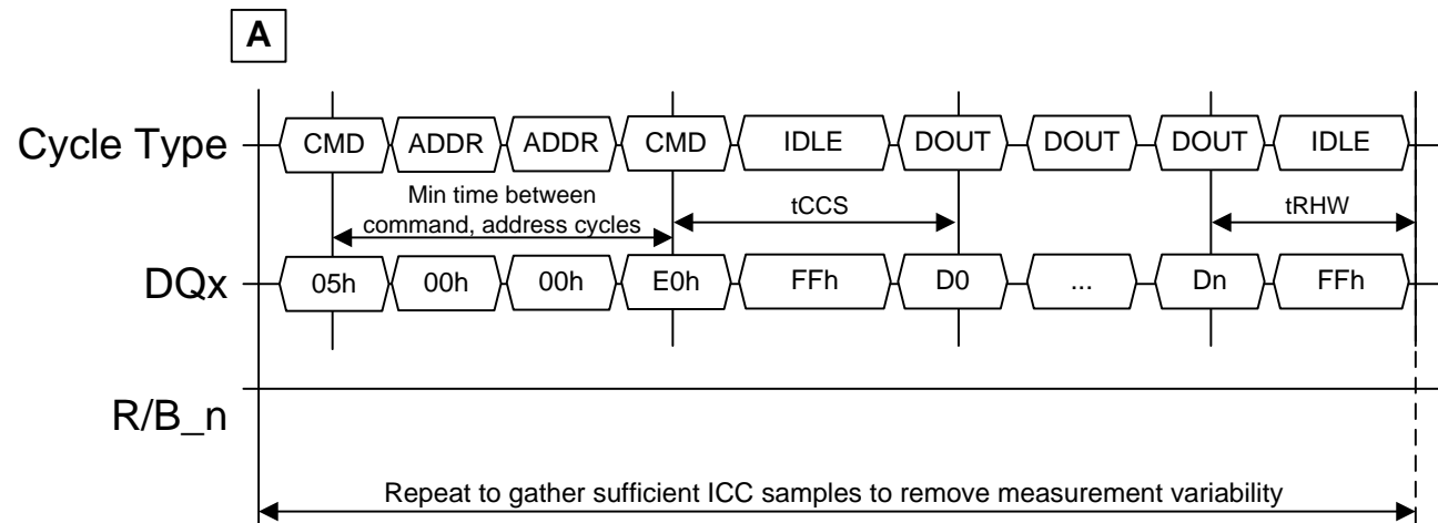
Figure 132 ICC4R and ICCQ4R measurement procedure
