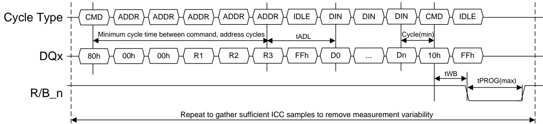
Figure 130 ICC2 measurement procedure
