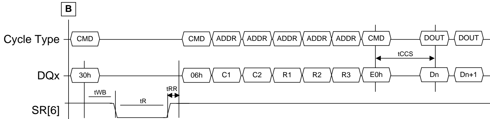
Figure 126 Multi-plane Read data output timing, continued from command issue
