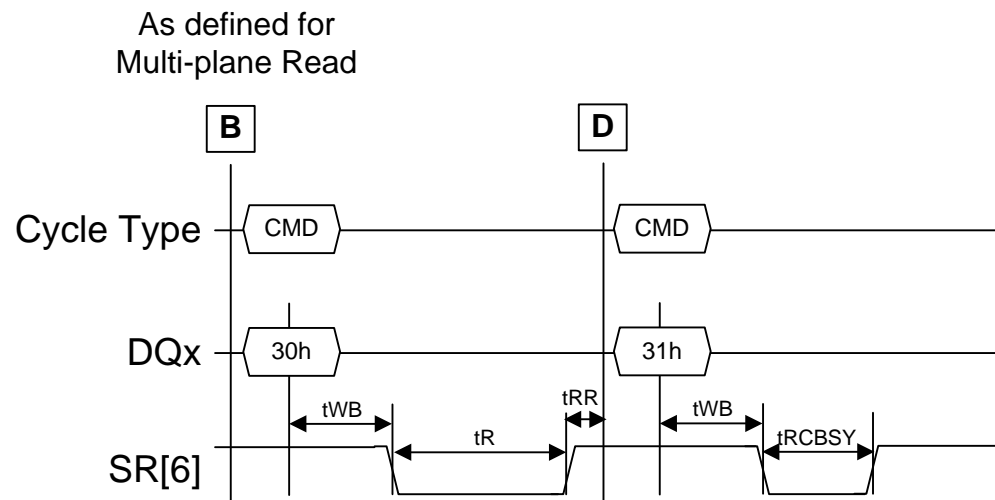
Figure 127 Multi-plane Read Cache Sequential command issue timing
