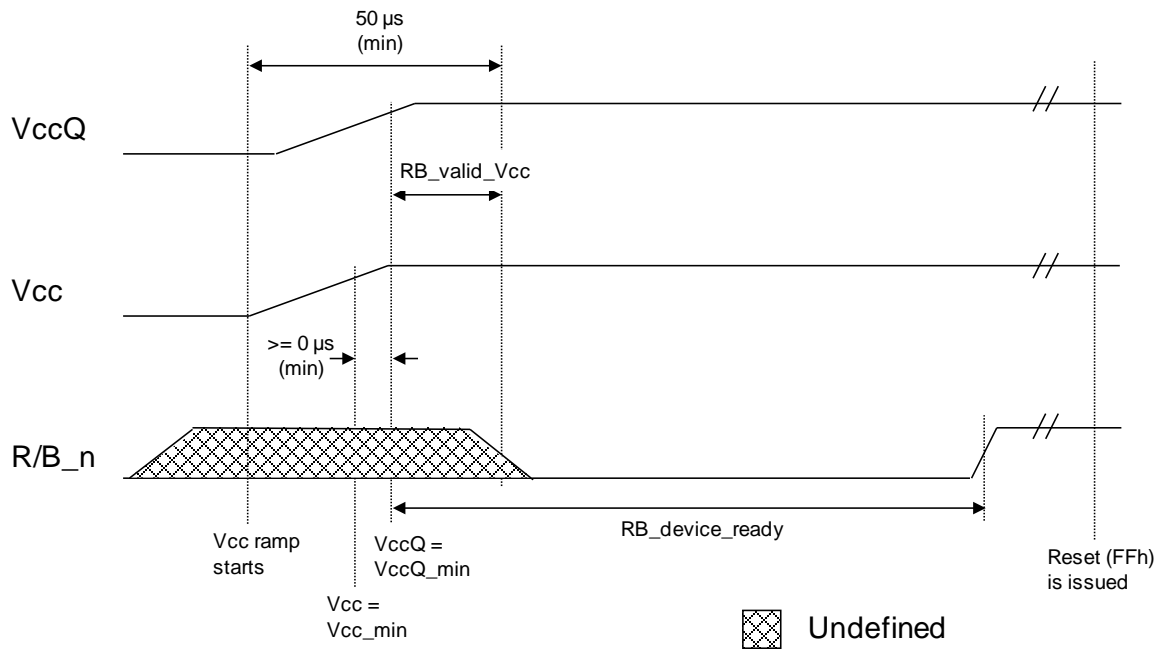
Figure 26 R/B n Power-On Behavior
