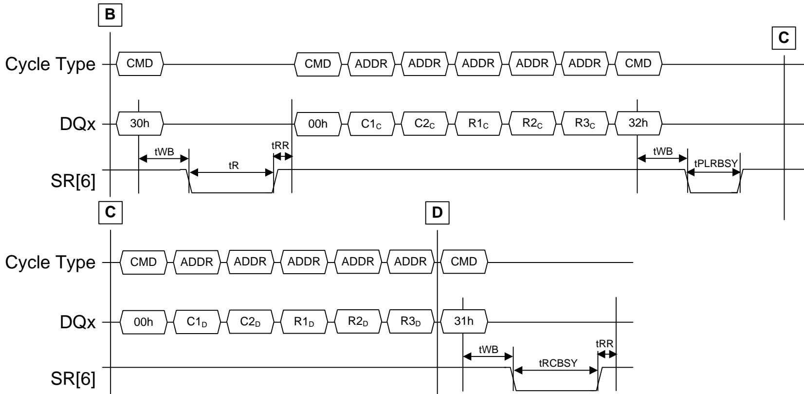
Figure 128 Multi-plane Read Cache Random command issue timing
