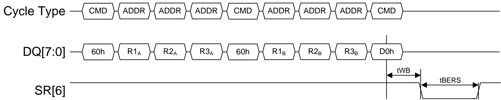
Figure 124 Multi-plane Block Erase timing, ONFI-JEDEC Joint Taskgroup primary definition
