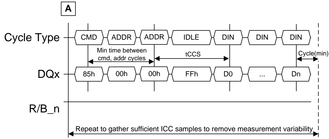
Figure 133 ICC4W measurement procedure
