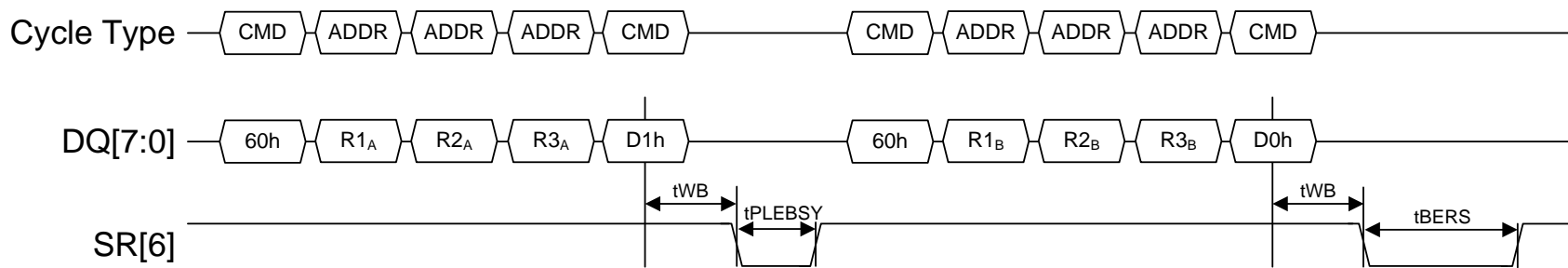
Figure 123 Multi-plane Block Erase timing
