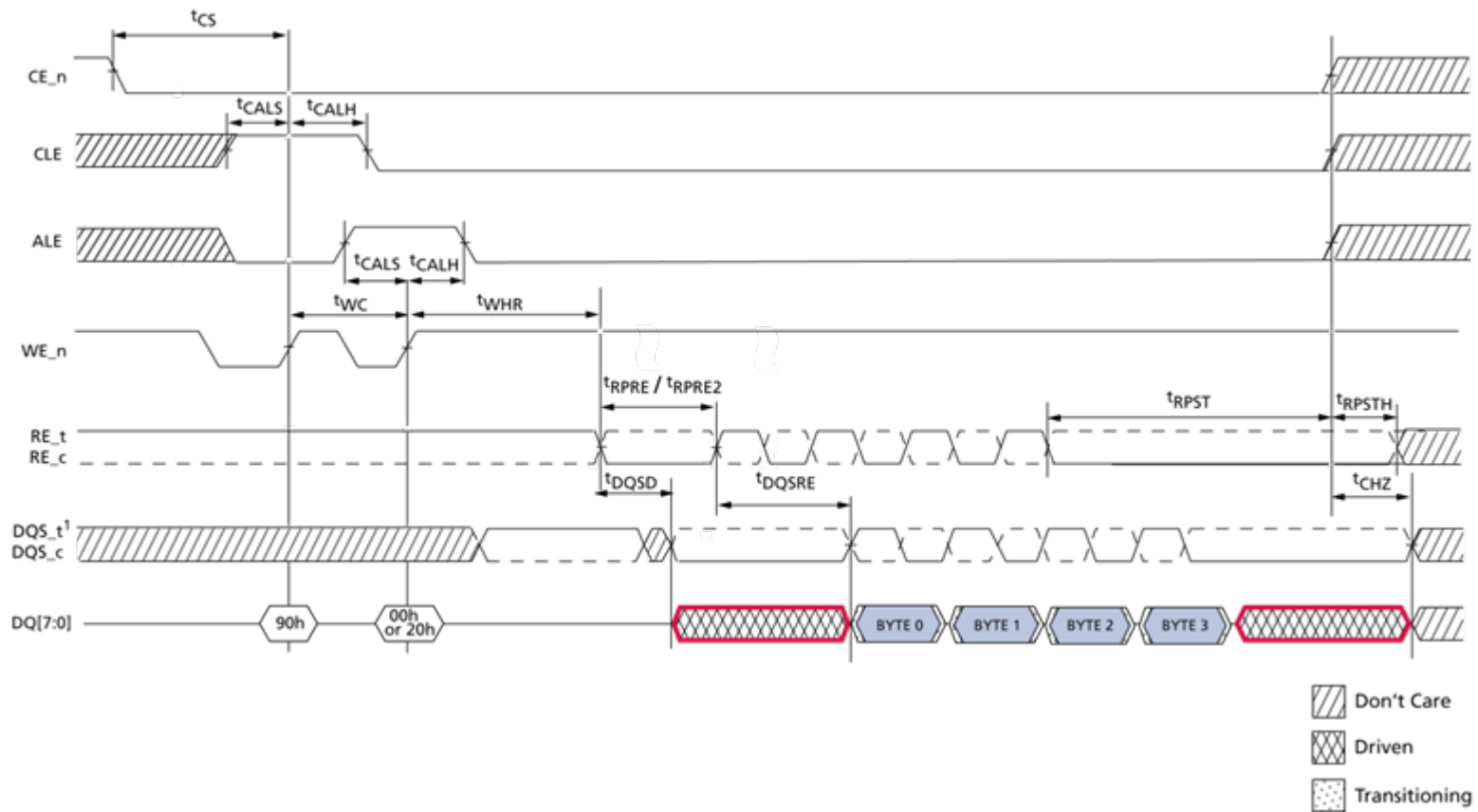
Figure 84 Read ID command using NV-DDR2 data interface
