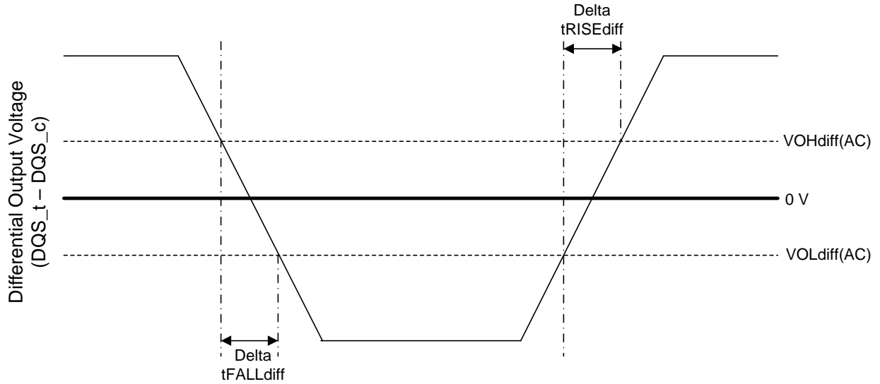
Figure 41 tRISEdiff and tFALLdiff Definition for Output Slew Rate, NV-DDR2 (differential)
