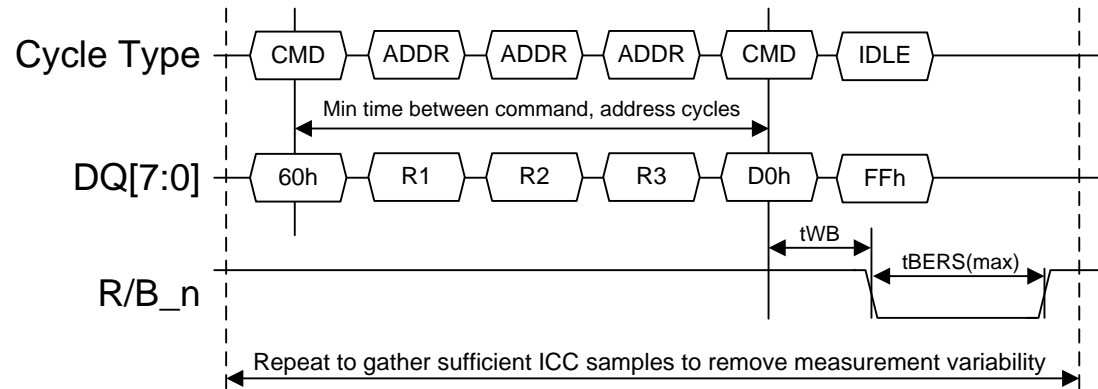
Figure 131 ICC3 measurement procedure
