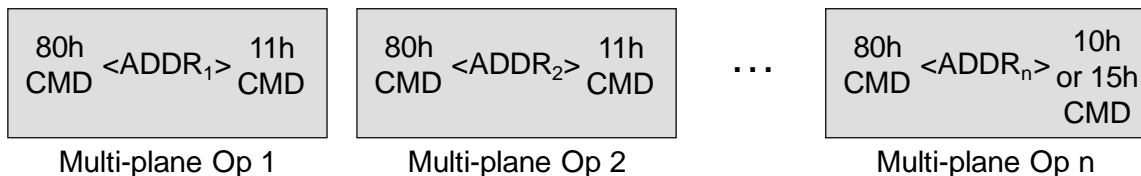
Figure 116 Multi-plane Program (Cache)
