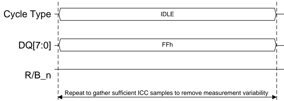
Figure 134 ICC5 measurement procedure
