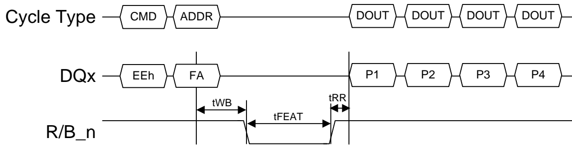
Figure 114 Get Features timing
