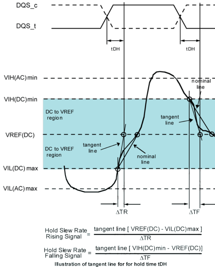
Figure 46 Tangent Line for Data Hold Time (tDH)
