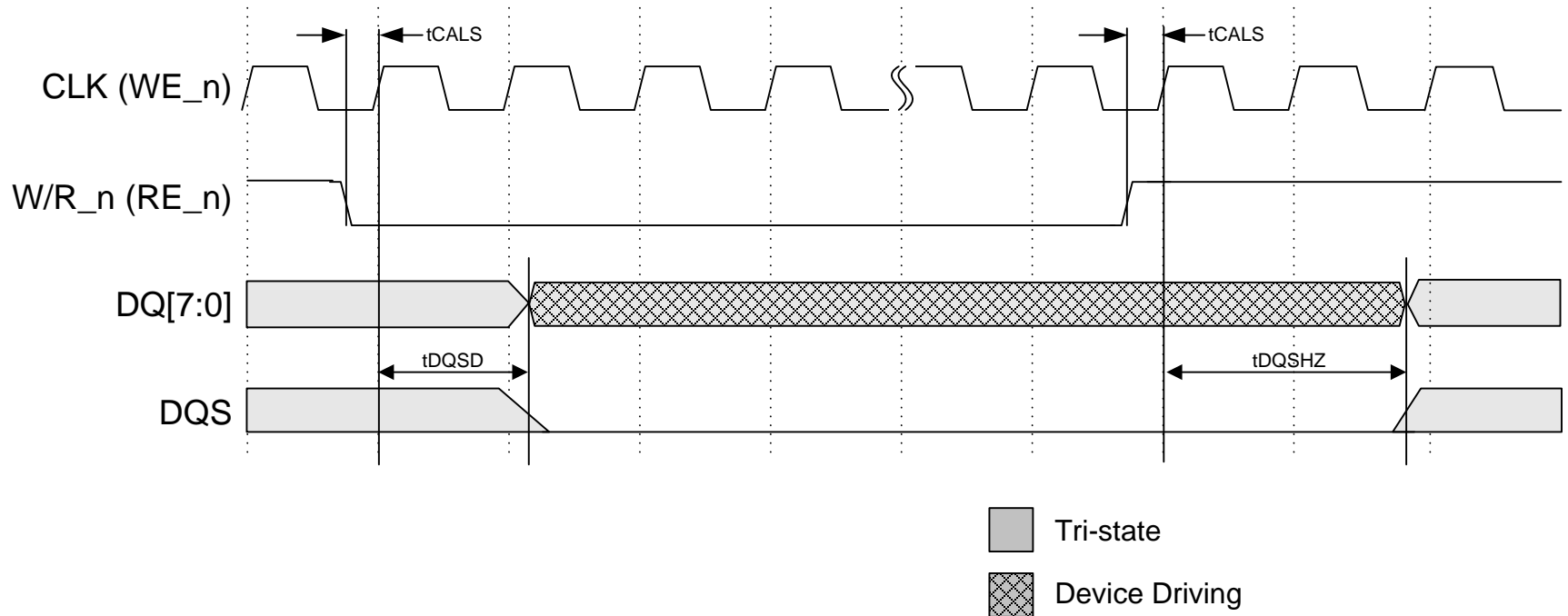
Figure 66 W/R_n timing
