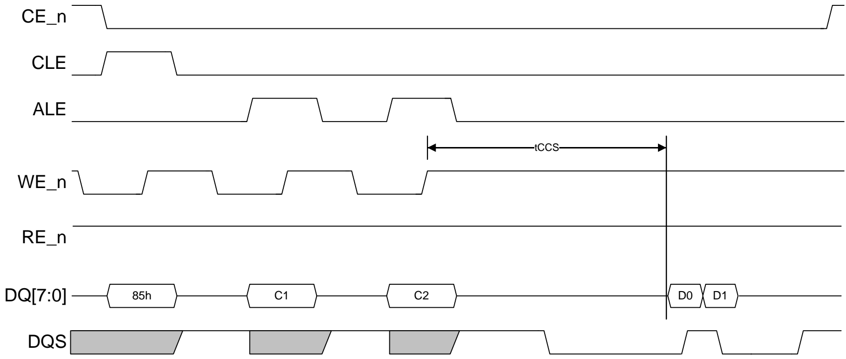
Figure 76 NV-DDR2 data interface command description
