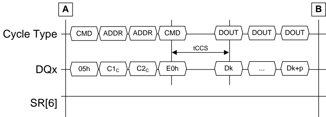
Figure 103 Small data moves, data modification
