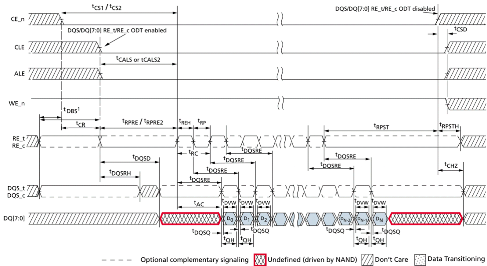
Figure 72 Data output cycle timing
