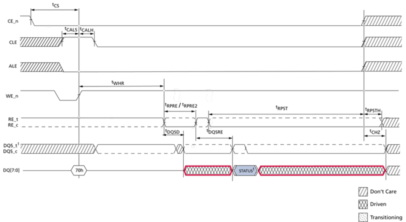
Figure 91 Read Status command using NV-DDR2 data interface
