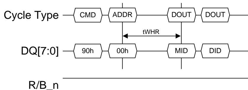
Figure 81 Read ID timing diagram for manufacturer ID
