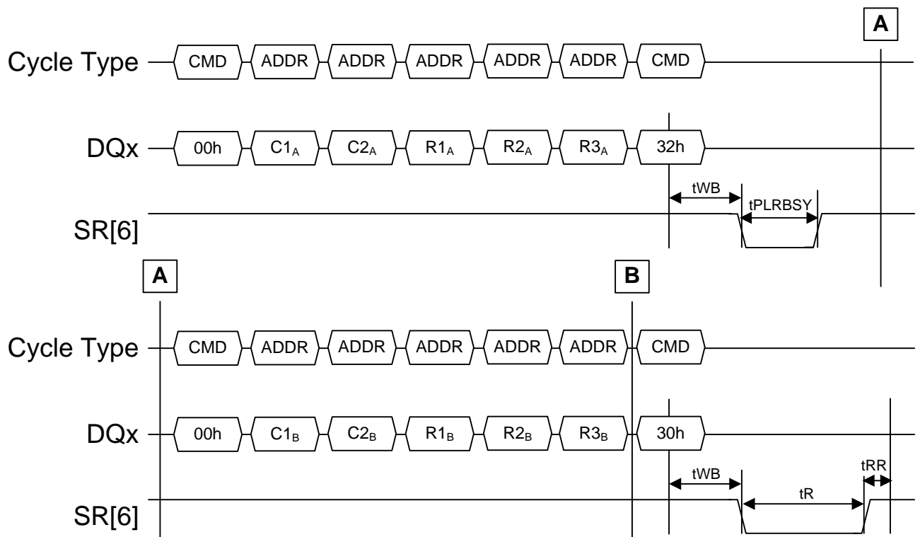
Figure 125 Multi-plane Read command issue timing
