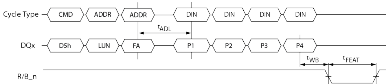
Figure 113 LUN Set Features timing
