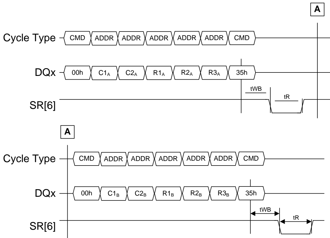
Figure 120 Non-multi-plane Copyback Read timing for multi-plane Copyback Program
