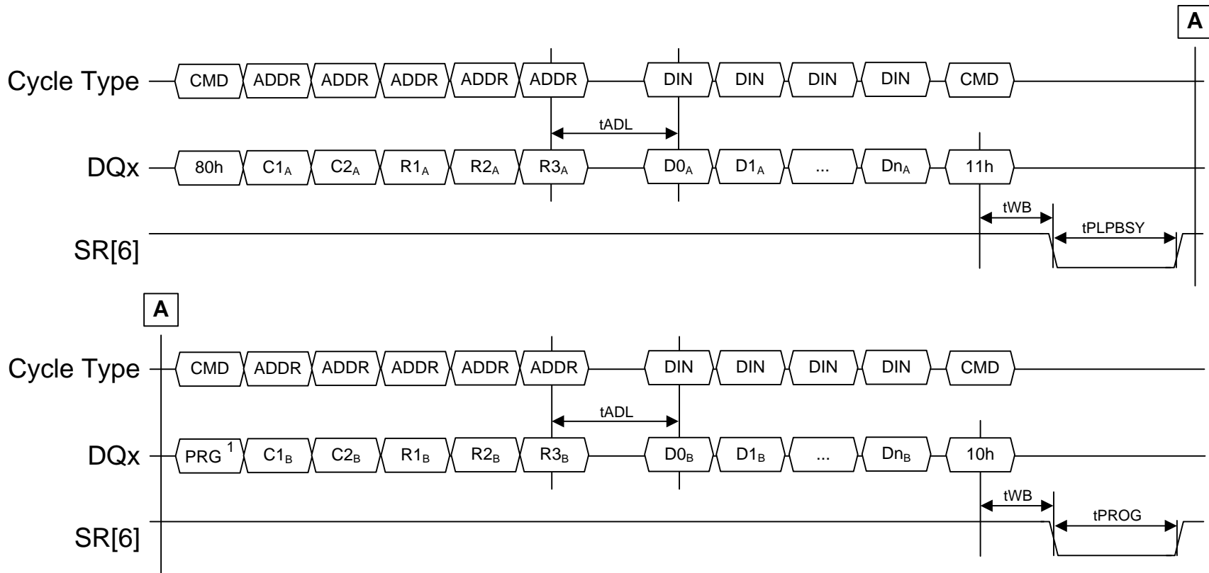
Figure 119 Multi-plane Page Program timing
