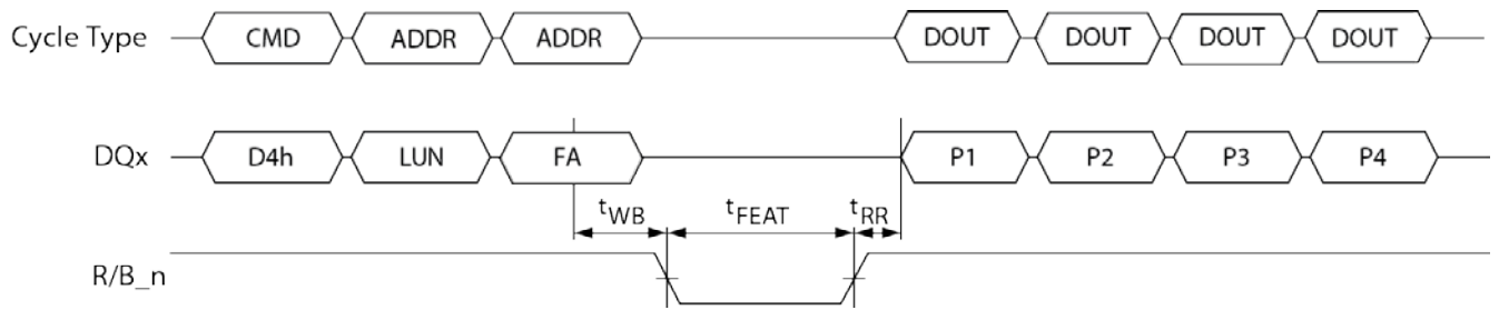
Figure 115 LUN Get Features timing
