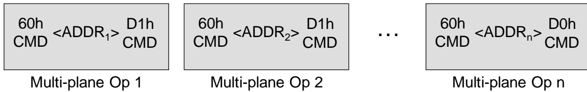
Figure 117 Multi-plane Erase
