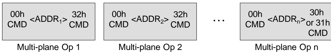
Figure 118 Multi-plane Read (Cache)
