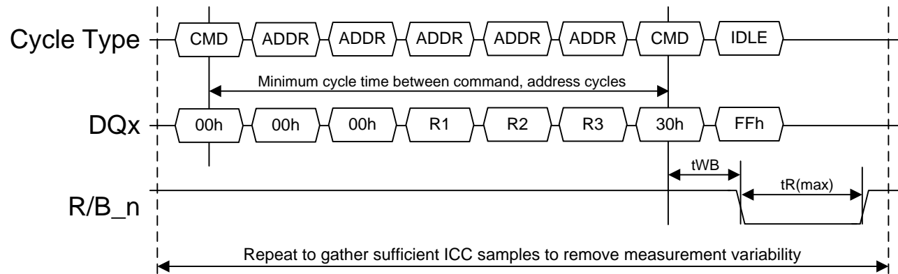
Figure 129 ICC1 measurement procedure
