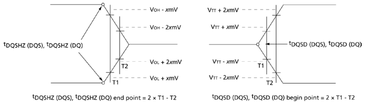
Figure 135 Two point method for measuring timing parameters with tri-state condition
