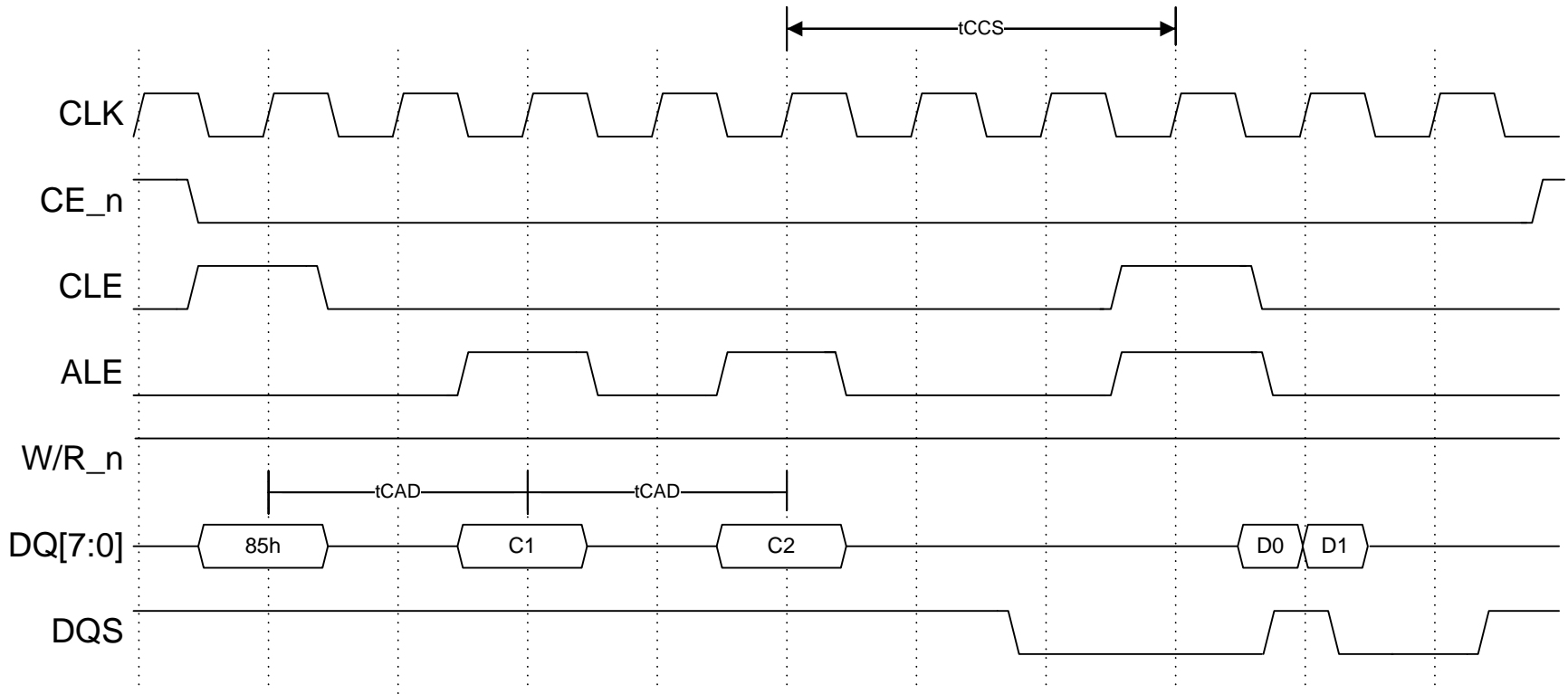
Figure 75 NV-DDR data interface command description
