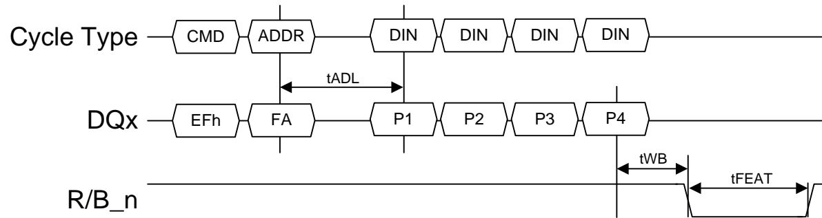
Figure 112 Set Features timing
