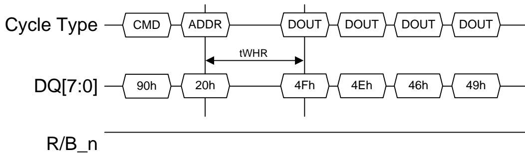
Figure 80 Read ID timing diagram for ONFI signature
