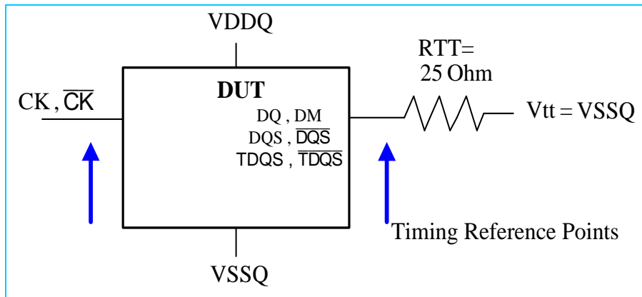
ODT Timing Reference Load
